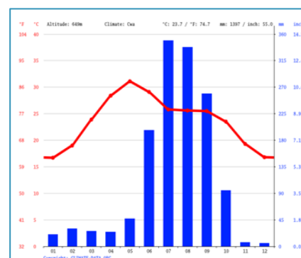
Diagramme climatique Inde (650m - Ranchi)
